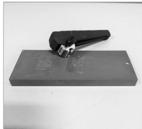
Figure 3 – 划格仪
